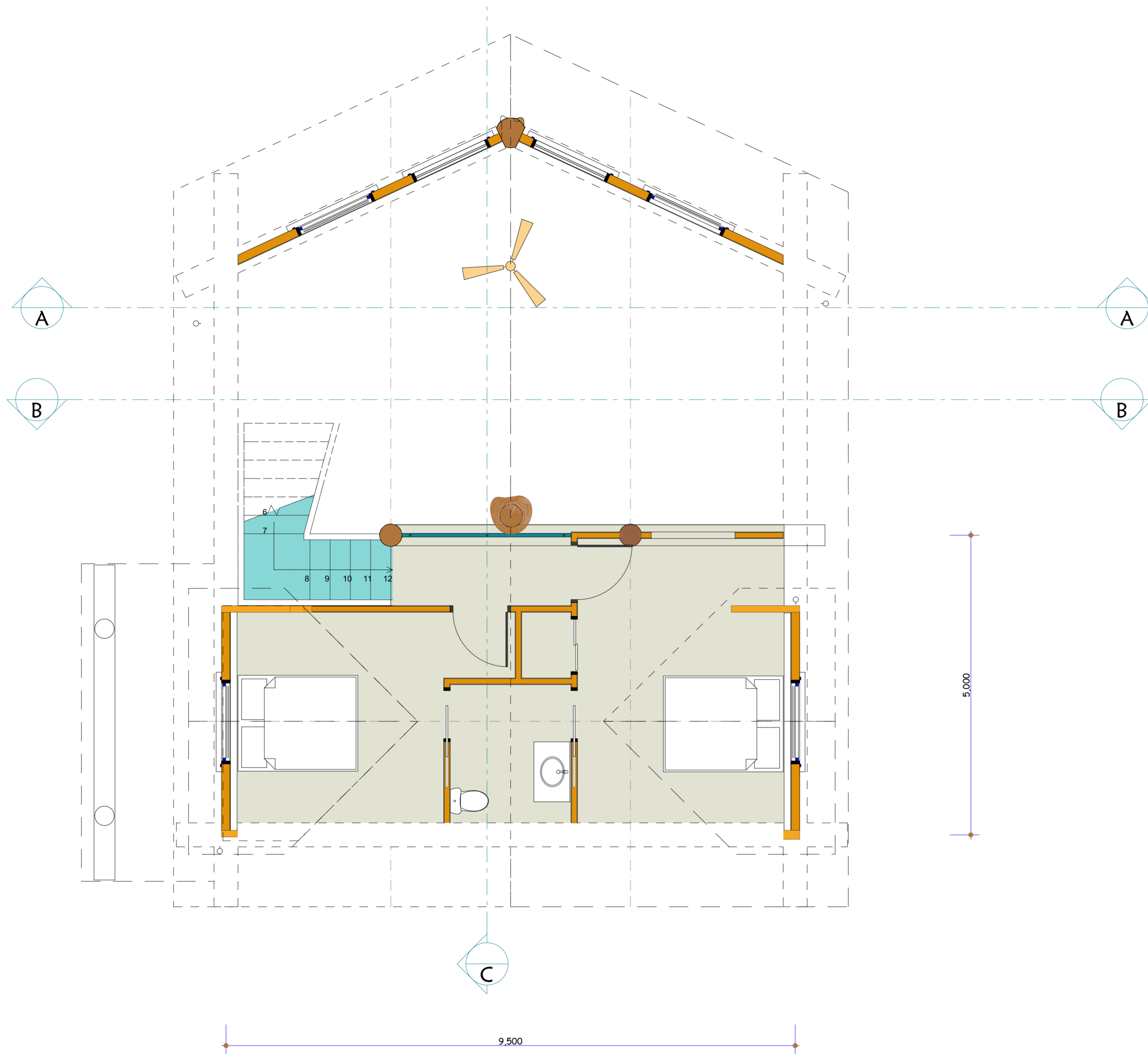
Loft Floor Plan 1:50
