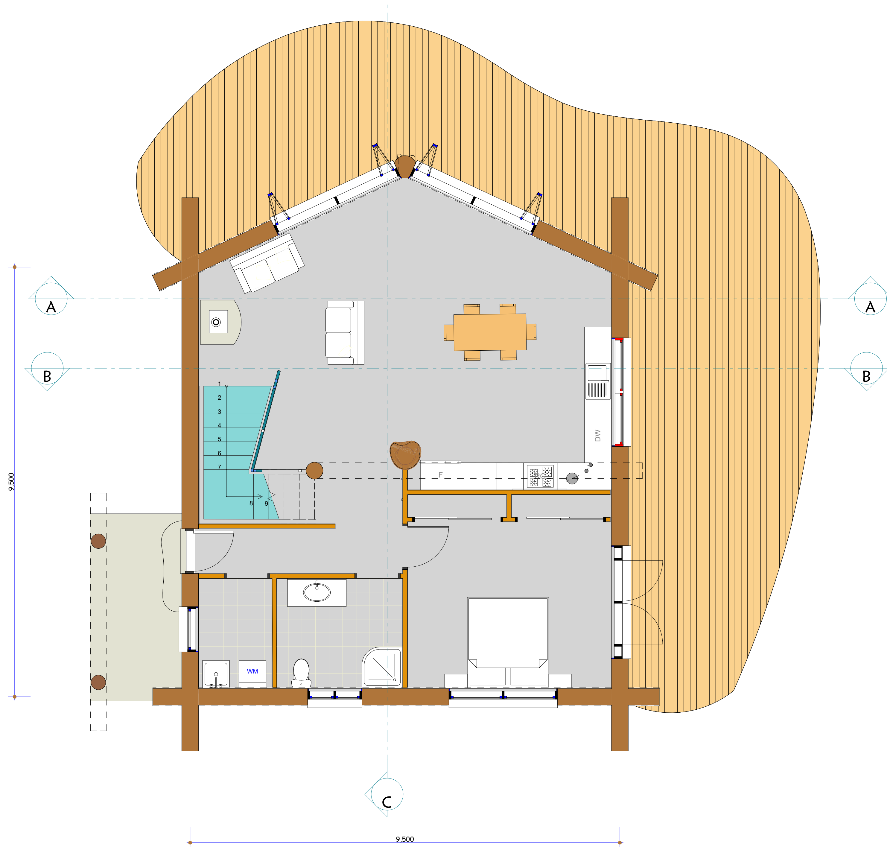
1 Ground Floor Plan 1:50
